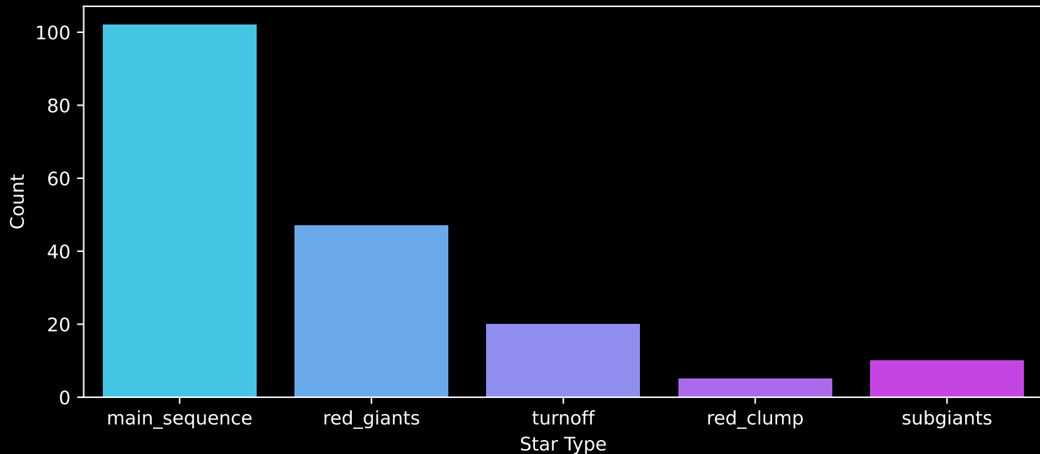
APOGEE DR17 Field: [190+60] Count plot of Star Type
