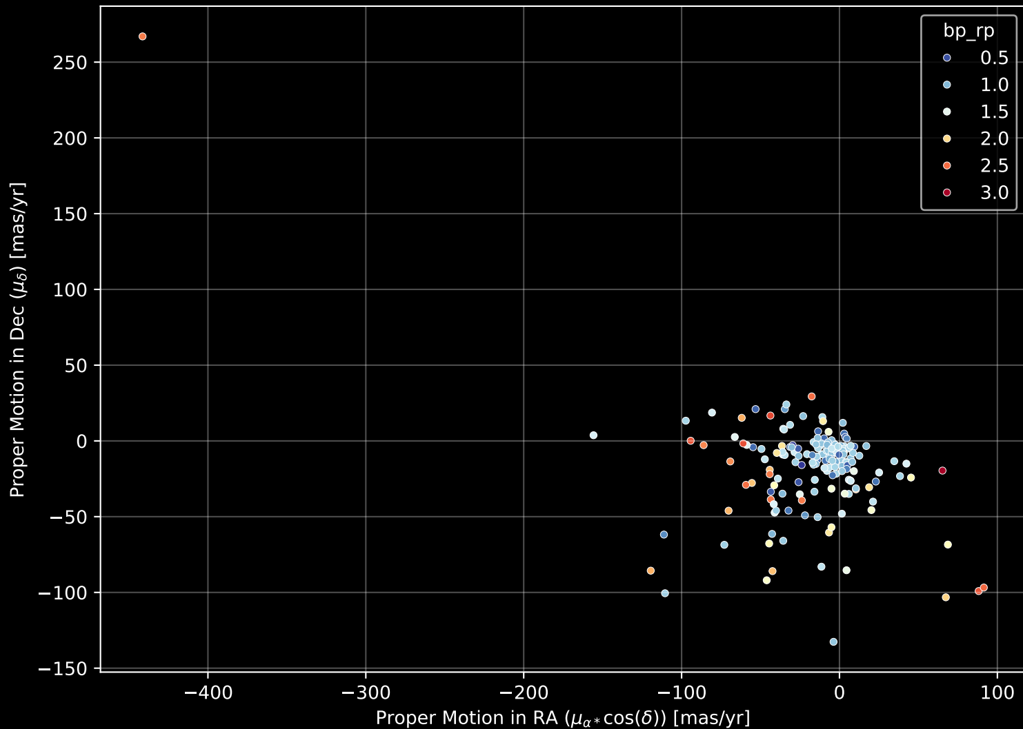
APOGEE DR17 Field: [190+60] Proper Motion Diagram (n= 184)
