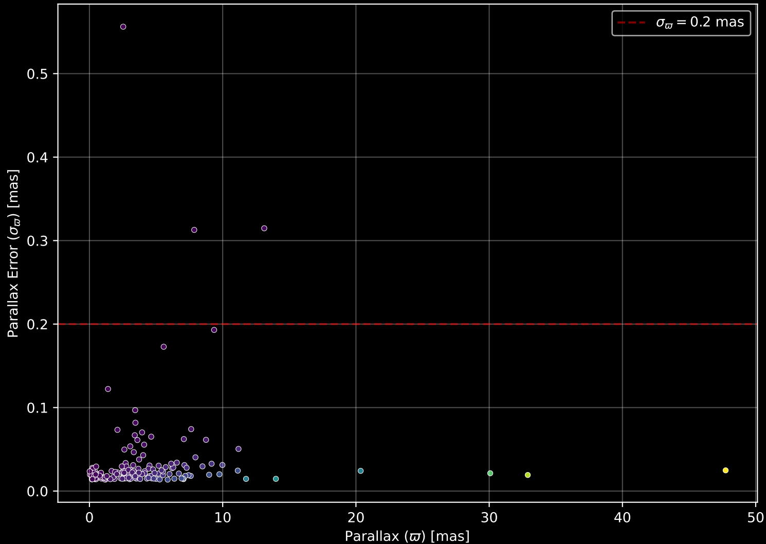
APOGEE DR17 Field: [190+60] Parallax Quality (n= 184)
