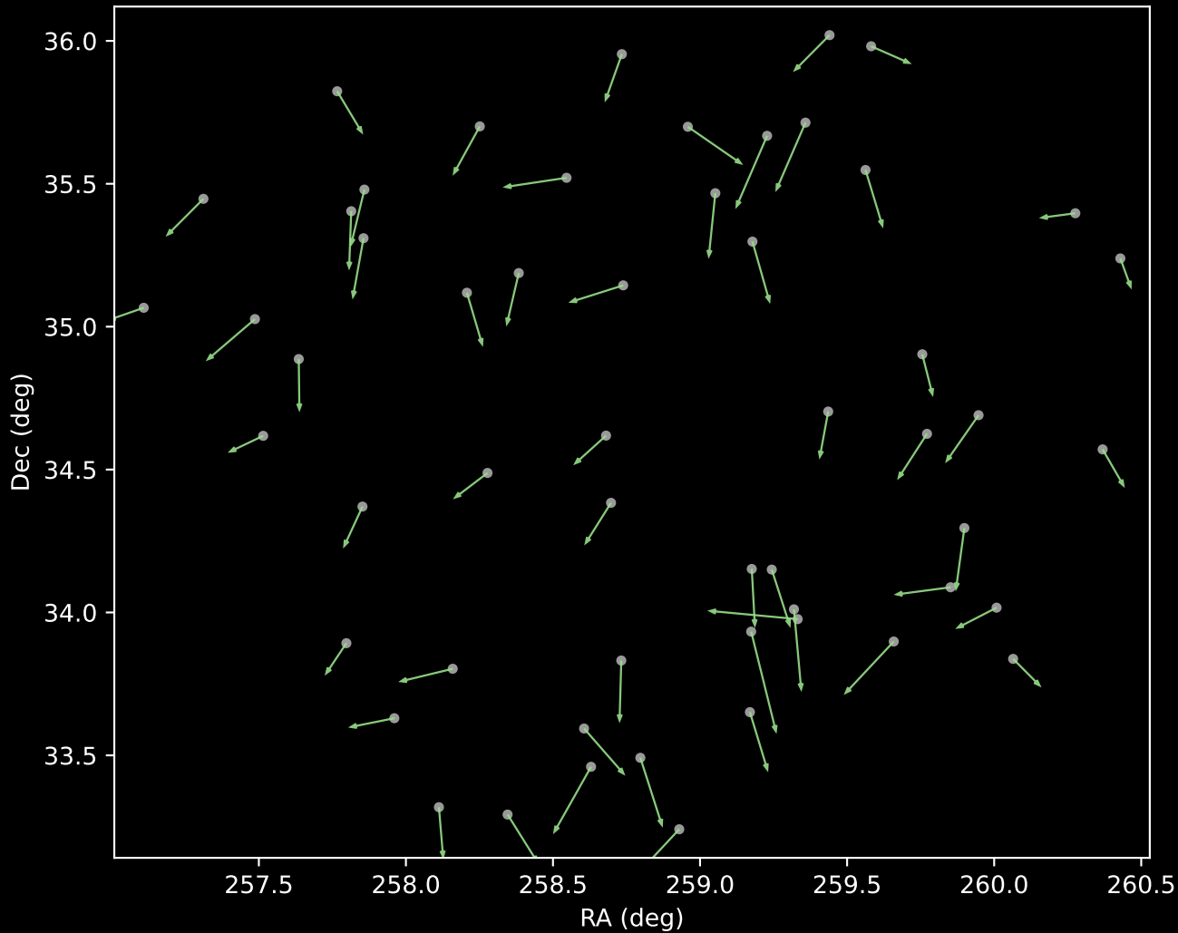
APOGEE DR17 Cluster 5 Proper Motion Vectors (n=55)
