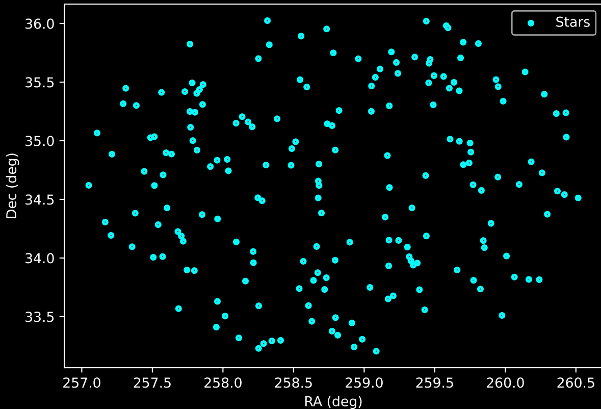
APOGEE DR17 Field: [190+60] Proper Motion Vectors for Gaia Star Field (n= 184)
