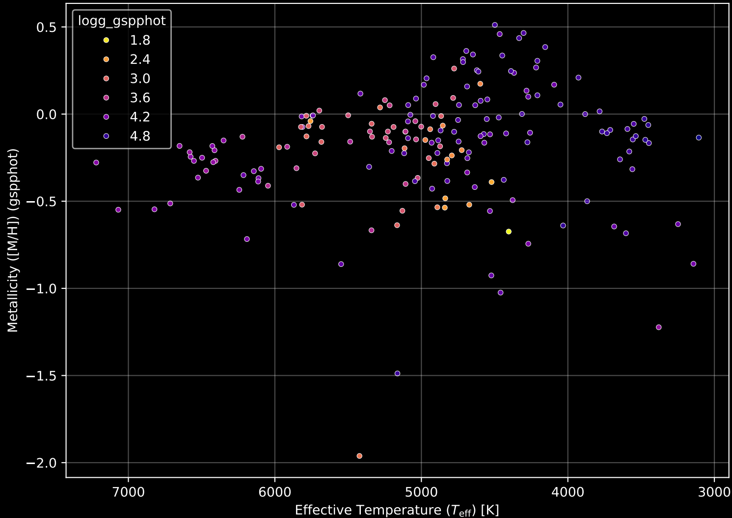
APOGEE DR17 Field: [190+60] Stellar Population Parameters (n= 184)
