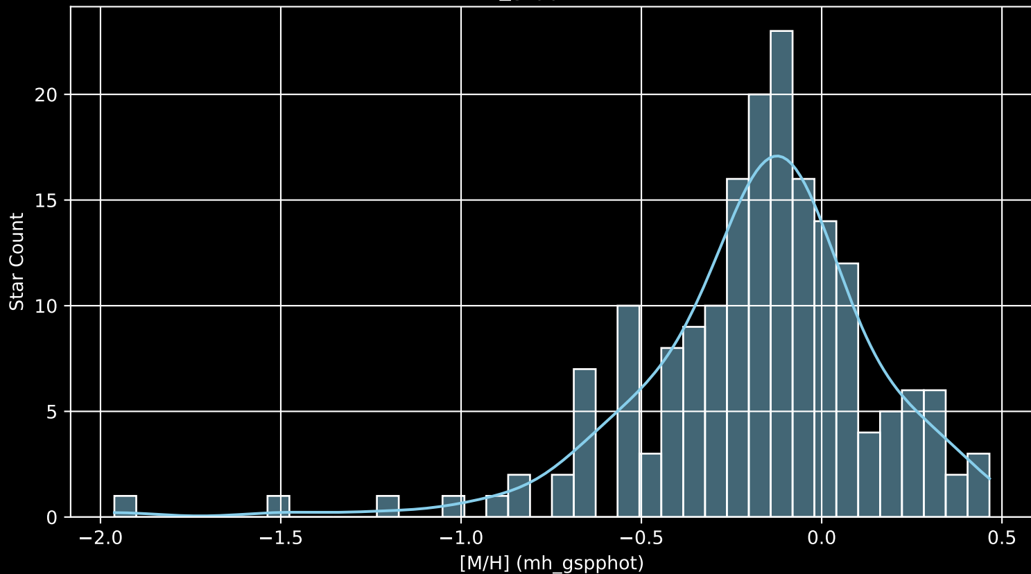
APOGEE DR17 Field: [190+60 [M/H] (mh_gspphot) (n= 183)
