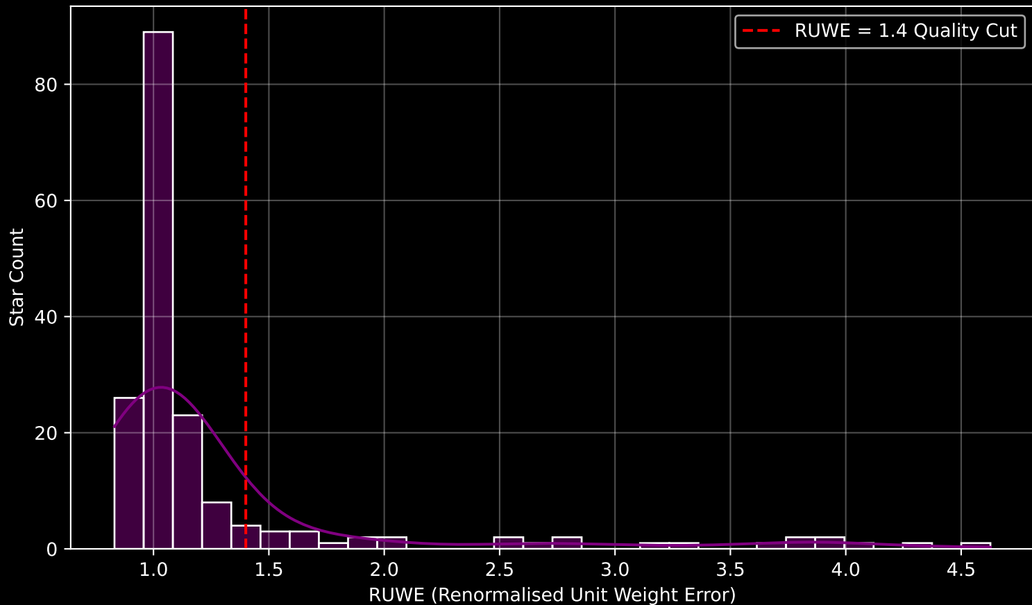
GAPOGEE DR17 Field [190+60] RUWE Distribution (n= 176)
